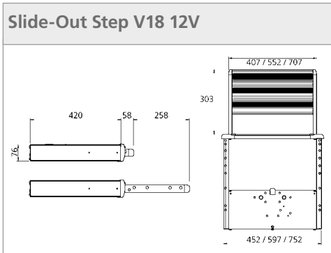
Slide-Out Step V18 12V
